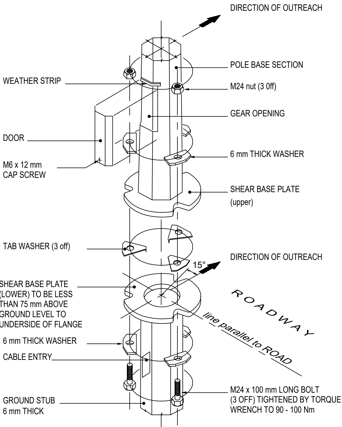
EXPLODED VIEW OF TYPICAL FRANGIBLE BASE ASSEMBLY
