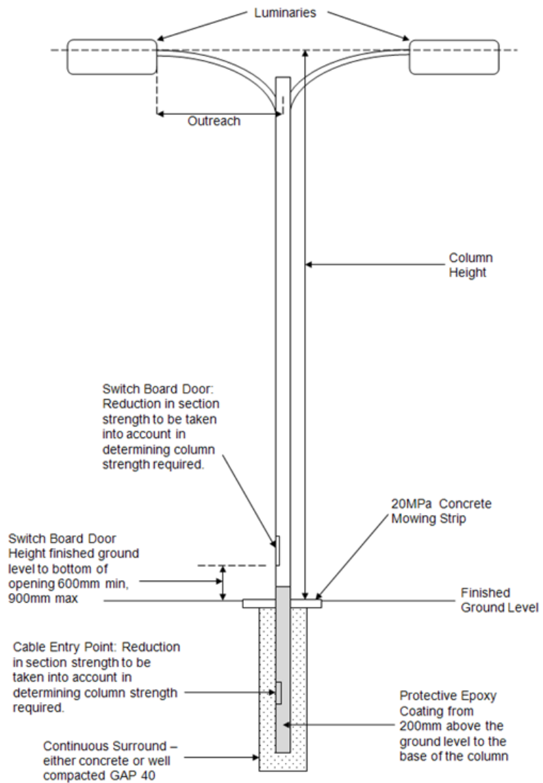
Figure A1: Parts of the lighting column
